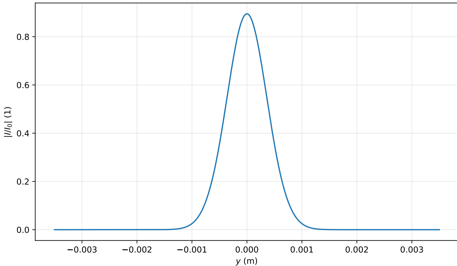
Intensity profile I(x=0, y, z=0.796)/I_0 , P_{in}=0.1P_{cr} , artificial time
